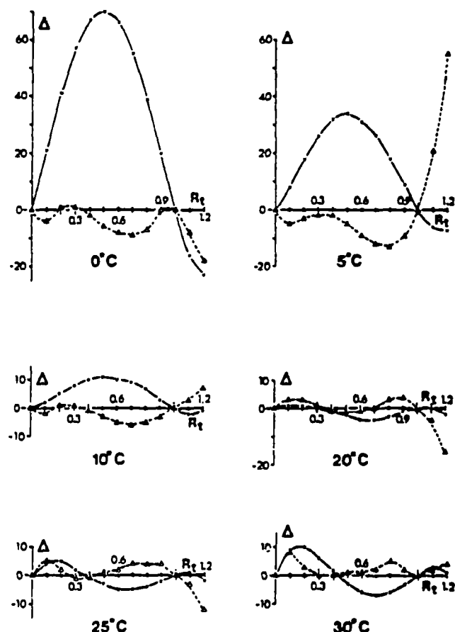
Fig. 5. Differences \Delta (\times 10^5) between \Delta_{15} calculated with polynomial 10 and those determined by Cox et al. (1967) (·) or by Brown and Allentoft (1966) ( \Delta ) versus conductivity ratio at different temperatures.
