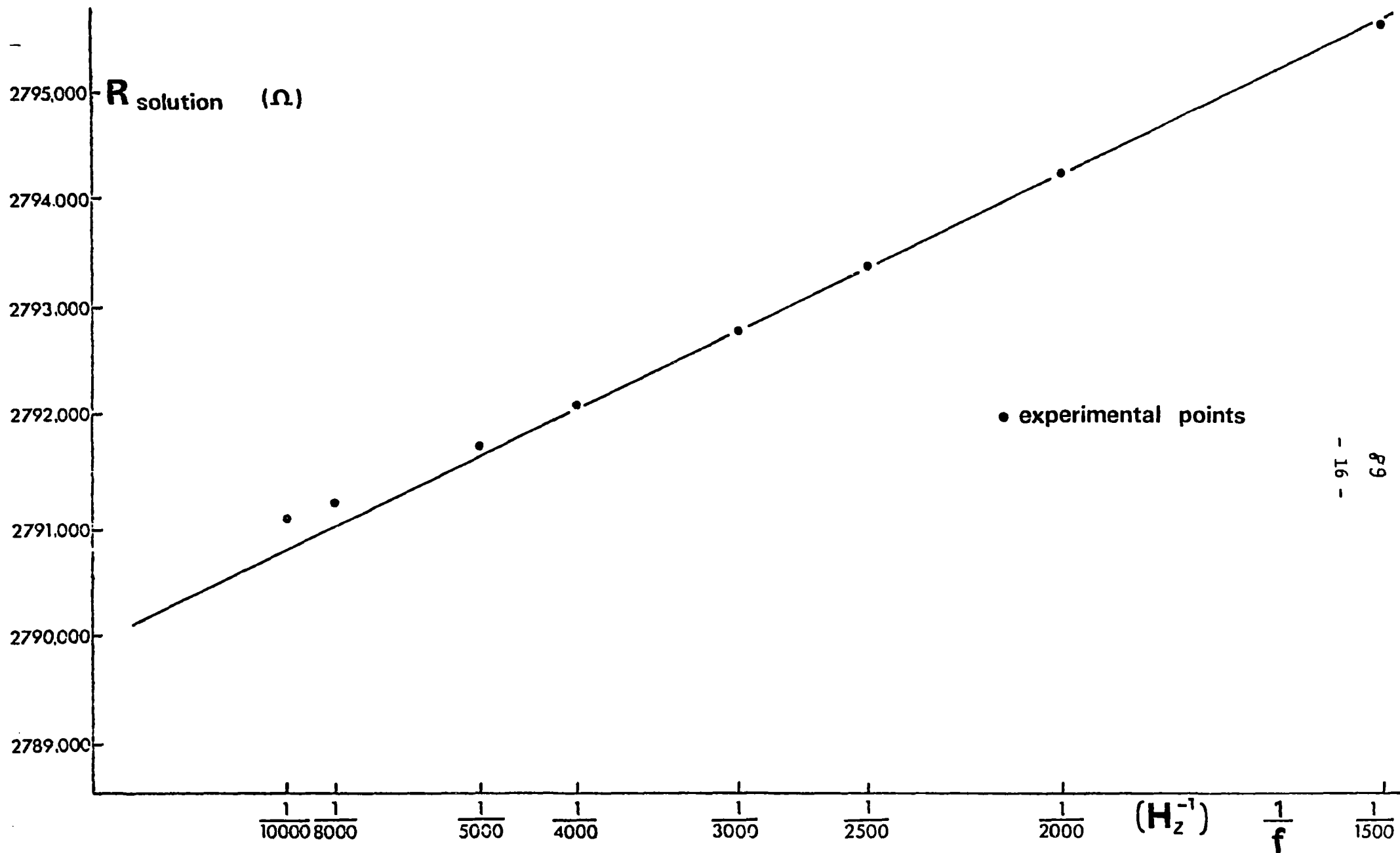
FIGURE 6 - STANDARD SEAWATER RESISTANCE VERSUS THE INVERSE OF THE CURRENT FREQUENCY
